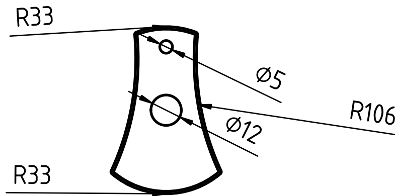
Crank Front
