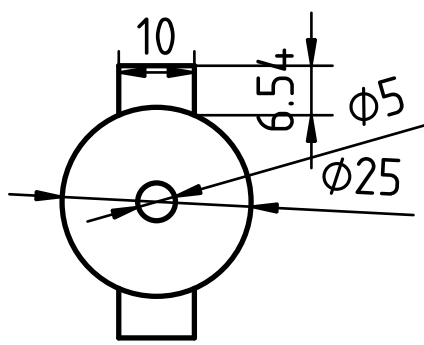
Slider rod front
