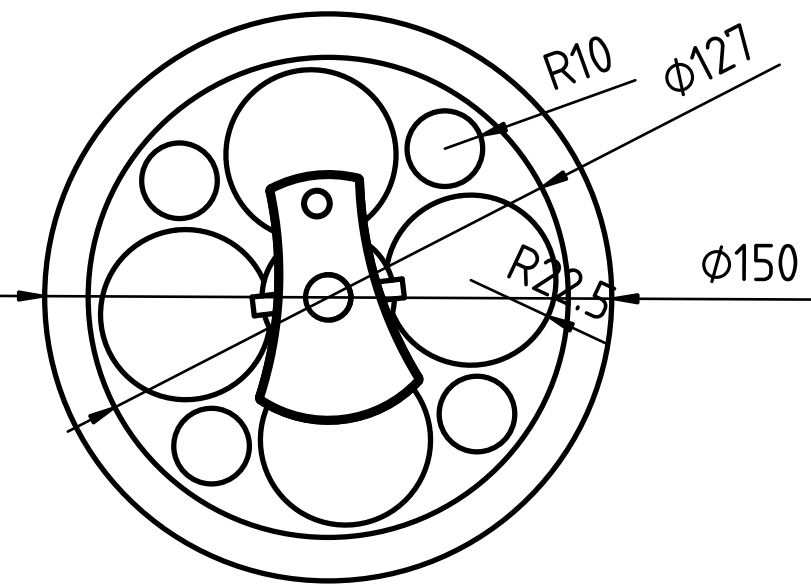
Flywheel Front
